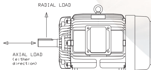
Axial Radial Loadings - Foot
