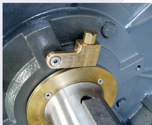
"Rotor Groundary Brush" fitted to D315 frame motor
