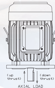
Axial Radial Loadings - Flange
